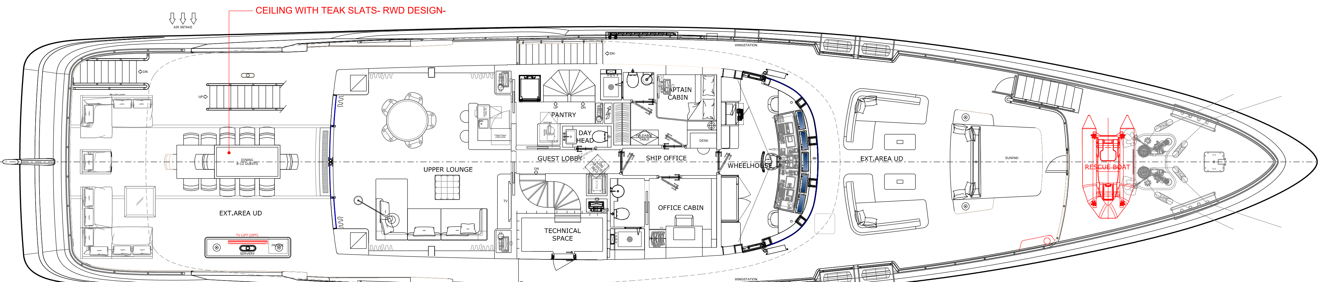
UPPER DECK
