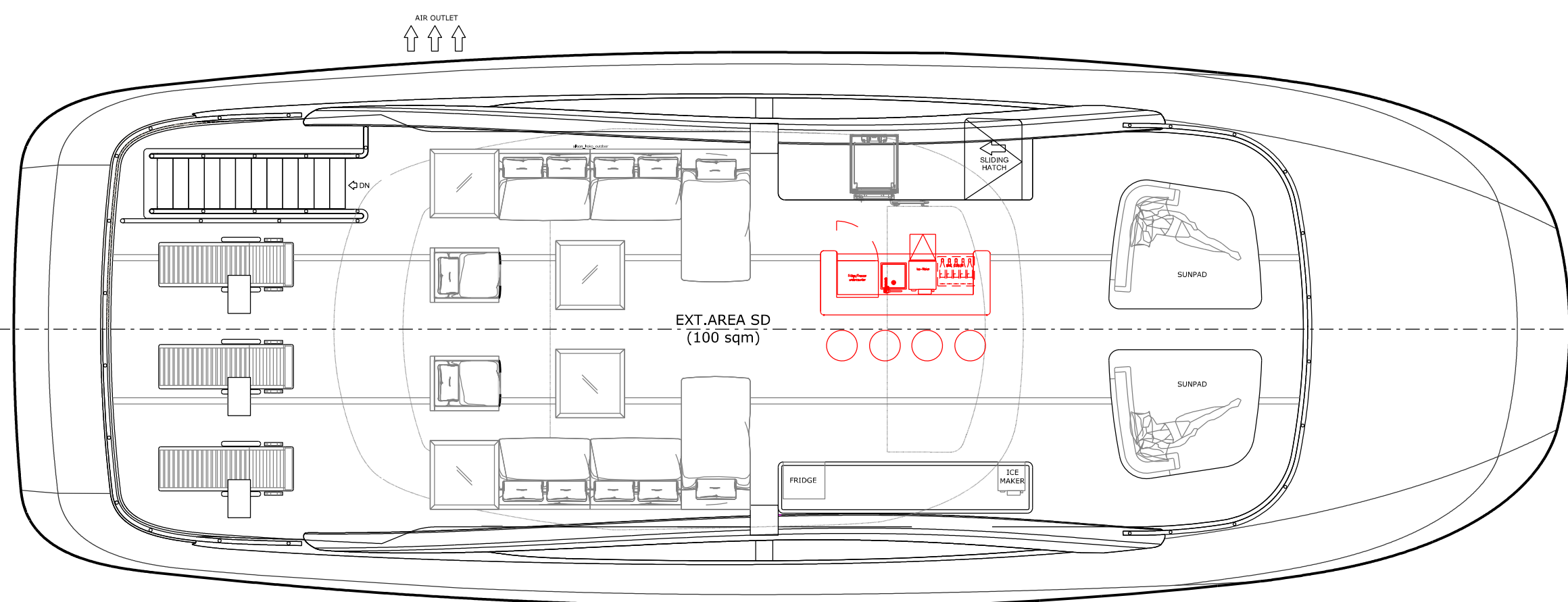
SUN DECK
