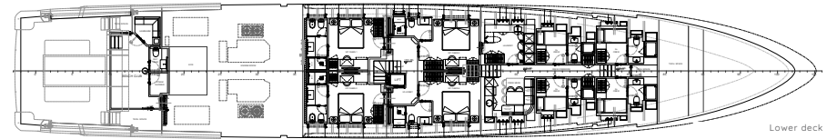
Lower deck
